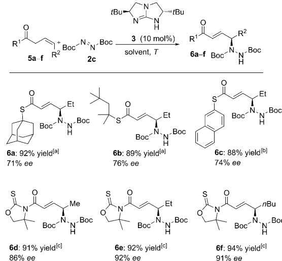
Scheme 2. \gamma -Selective direct allylic amination of ( Z )- \beta,\gamma -unsaturated thioesters and acetyloxazolidinethiones with di- tert -butyl azodicarboxylate. [a] Et 2 O, –20 °C, yield of isolated product after 24 h. [b] MTBE, –50 °C, yield of isolated product after 4 h. [c] n -Hexane, RT, yield of isolated product after 36 h.
